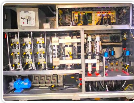
Inside view of Traction converter
